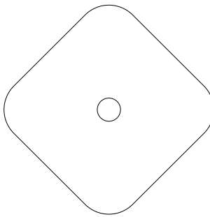
DETAIL 4 SCALE 1:1 □ 1 1/4"
